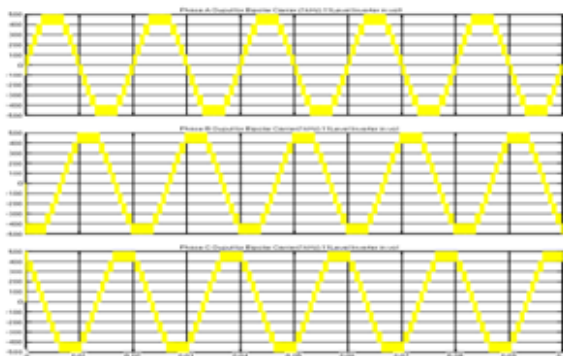
Fig 11: Voltage of 11 level 3 Phase CHB across load terminals with Bipolar SPWM switching When mIndex = 1
