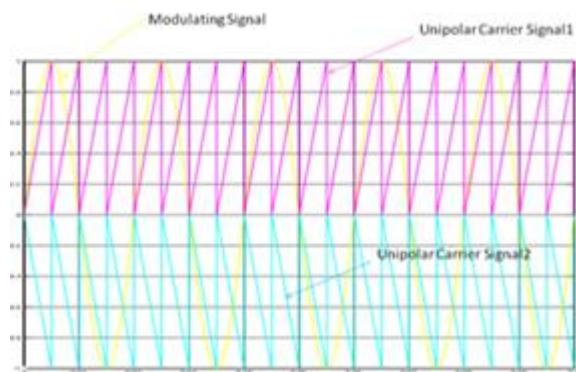
Fig 3: Unipolar switching sequence generation.
