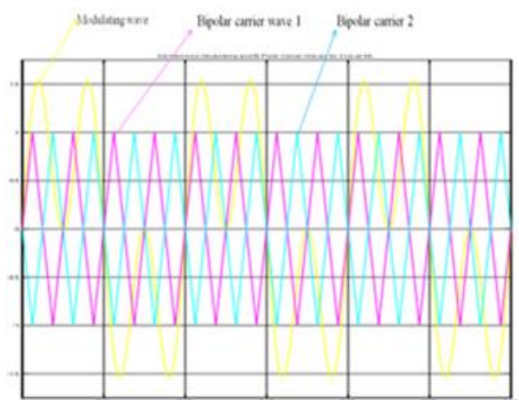
Fig 10: Bipolar 3rd Harmonic Signals
