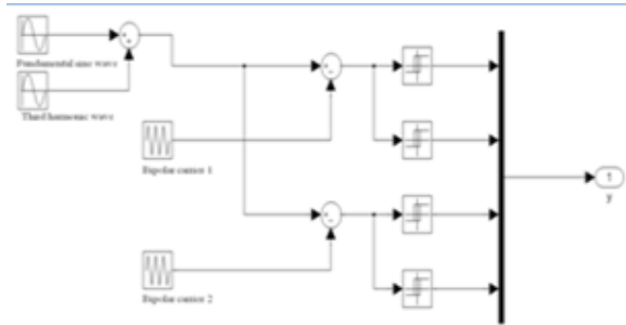
Fig 7: Unipolar switching sequence With 3rd Harmonic modulating signal.
