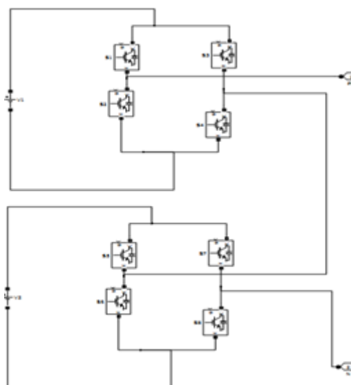
Fig 1: Cascaded H Bridge based Multilevel Inverter
