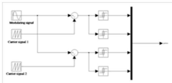
Fig 4: Unipolar Switching signals.
