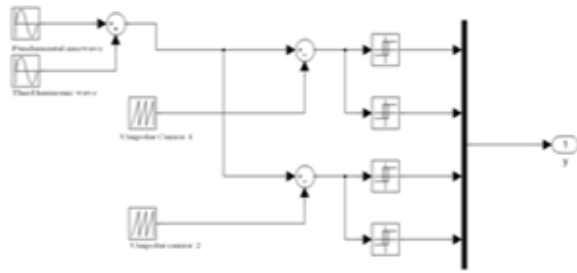
Fig 9: Bipolar switching sequence With 3 rd Harmonic modulating signal.
