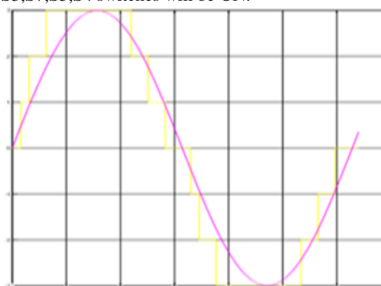
Fig 2: Output of a Seven Level Inverter.
