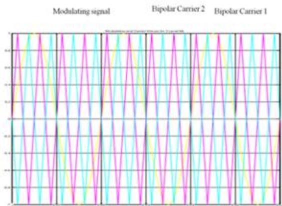
Fig 5: Bipolar switching sequence generation
